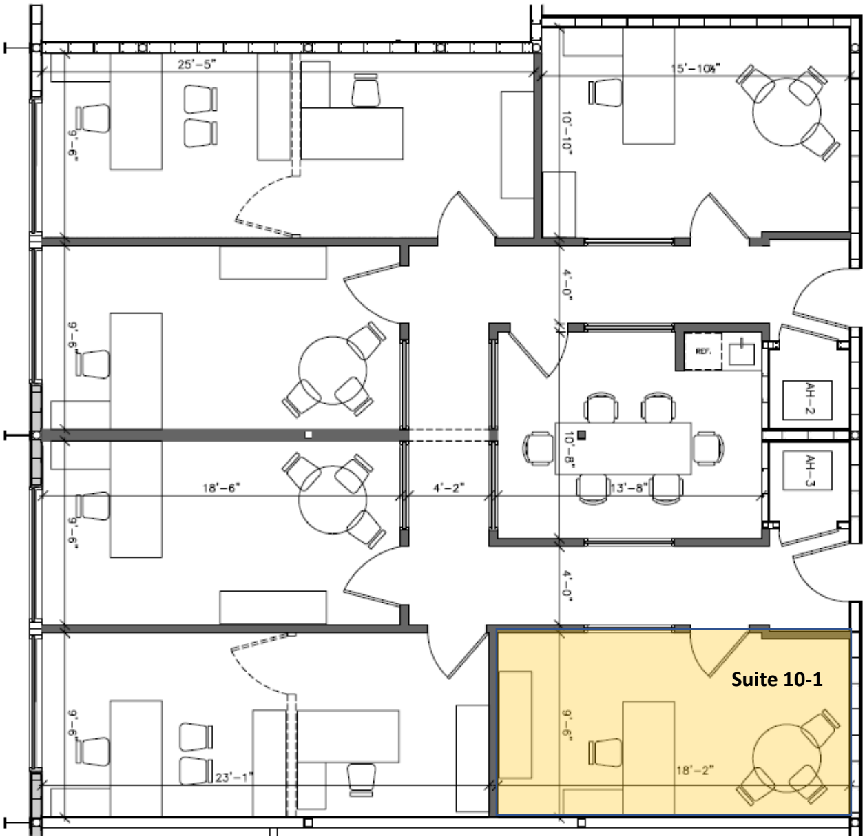
1 PROPOSED CENTRAL SUITES FLOOR PLAN SCALE: 3/8" = 1'-0"
